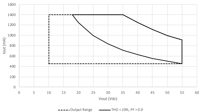
PLS-A50W-14-55 Operating Envelope
